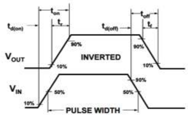
Figure8. Switching wave
