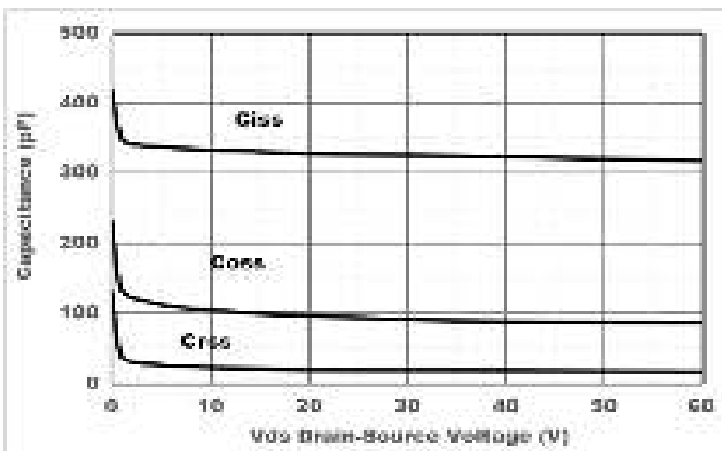
Figure3. Capacitance Characteristics
