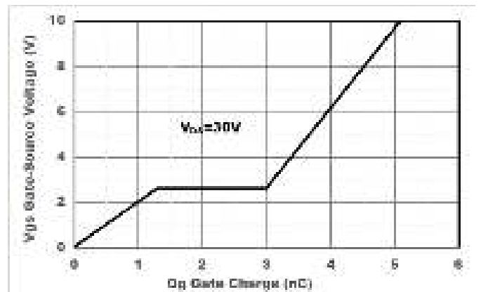
Figure4. Gate Charge
